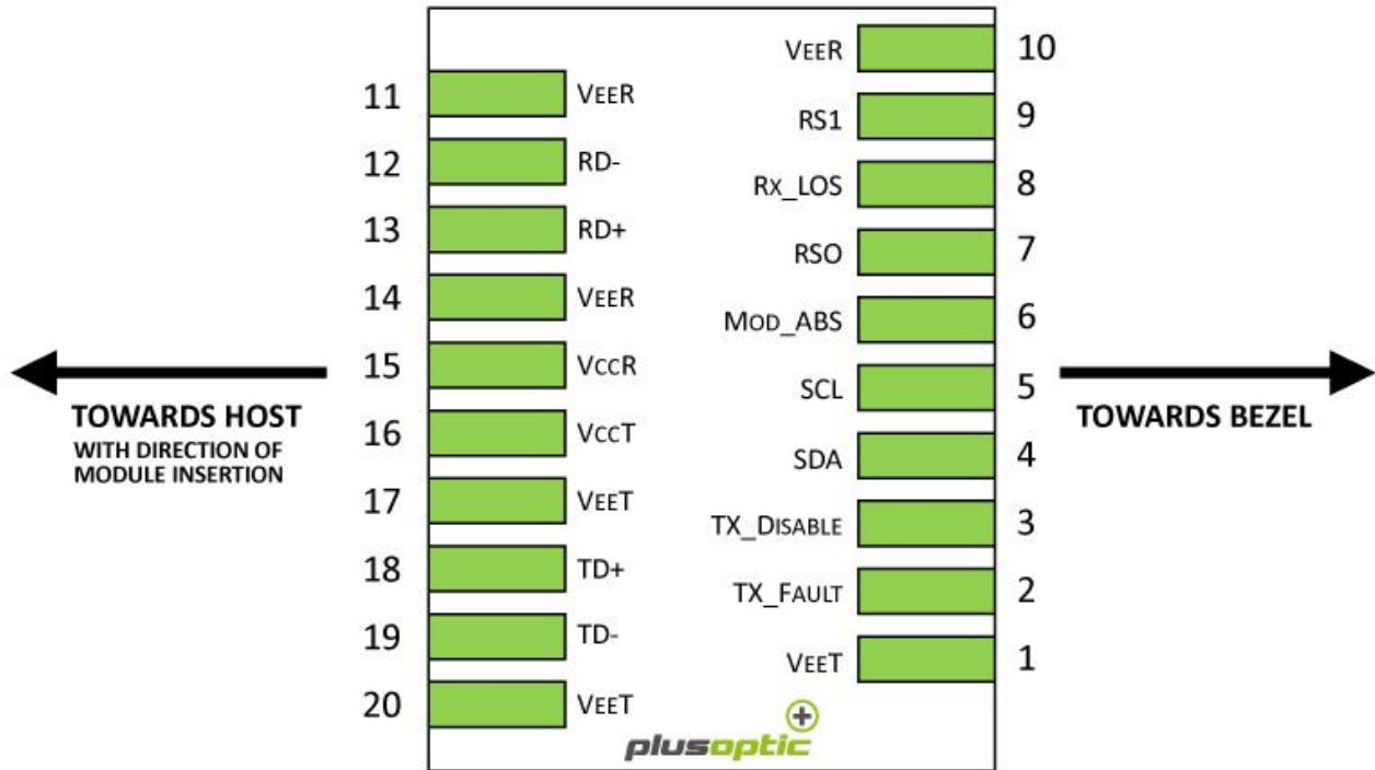
Figure 2: Pin-out of Connector Block on Host Board
